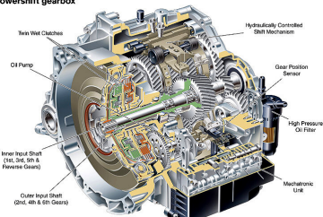
Powershift gearbox
