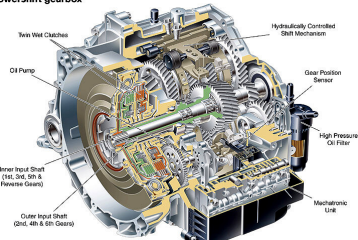
Powershift gearbox
